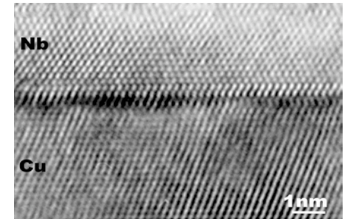
5 nm layer thickness Cu-Nb multilayer
