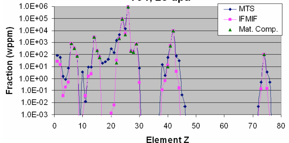
T91, 25 dpa
