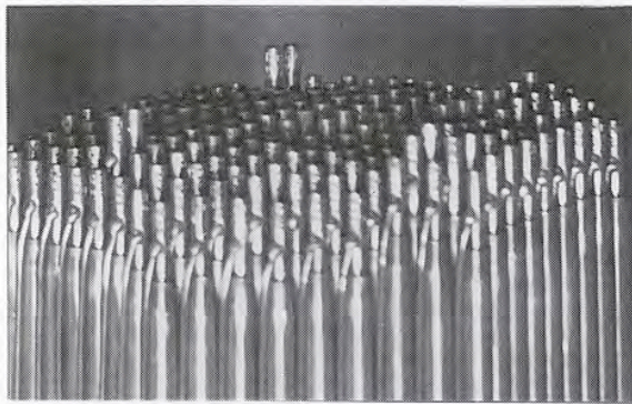
D9 irradiated to 2.1 \times 10^{23} ( E > 0.1 \text{ MeV} )*
