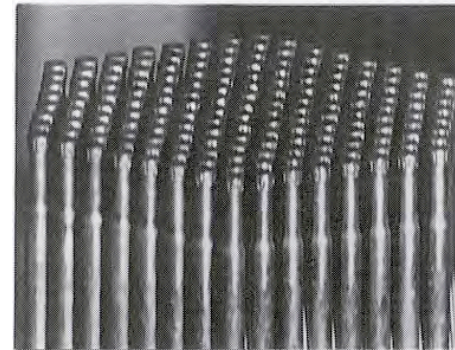
HT9 irradiated to 1.9 \times 10^{23} ( E > 0.1 \text{ MeV} )*
